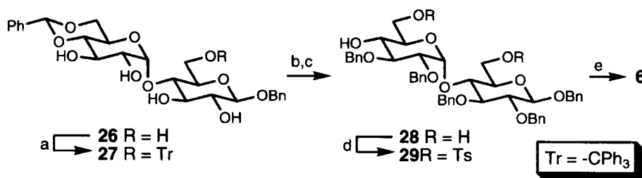
Fig. 4. Alternative synthesis of monohydroxy derivative of \alpha -D-quinovosyl-(1 \rightarrow 4)-D-quinovose. a) TrCl/Pyridine, \Delta ; b) BnBr, NaH/DMF, 0 °C; c) aq AcOH (80%), \Delta ; d) TsCl/Pyridine, 0 °C \rightarrow room temp; e) LiAlH 4 /Et 2 O, \Delta ; f) RhCl(Ph_3P)_3/EtOH-PhH-H_2O , \Delta ; g) dil HCl/Me 2 CO, \Delta .
